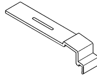
Window sill holder RS 40 for brick work
